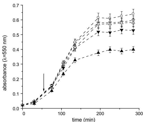
Figure 5. Growth delay curves of E. coli incubated with 10\ \mu\text{M} of ZnPc 1 (▼) and ZnPc 2 (▲) and exposed to different irradiation times with visible light in 10% w/v TS broth at 37\ ^\circ\text{C} . The arrow marks the time point where the appropriate concentration of phthalocyanine was added. Control culture untreated irradiated (○), treated with 10\ \mu\text{M} of ZnPc 1 (▽) and ZnPc 2 (△) and not irradiated. Values represent means \pm standard deviation of three separate experiments.
