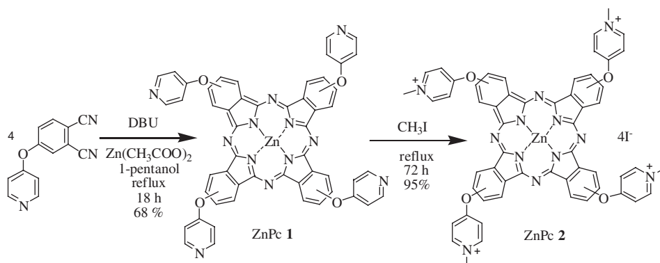
Scheme 2. Synthesis of ZnPcs 1 and 2.
