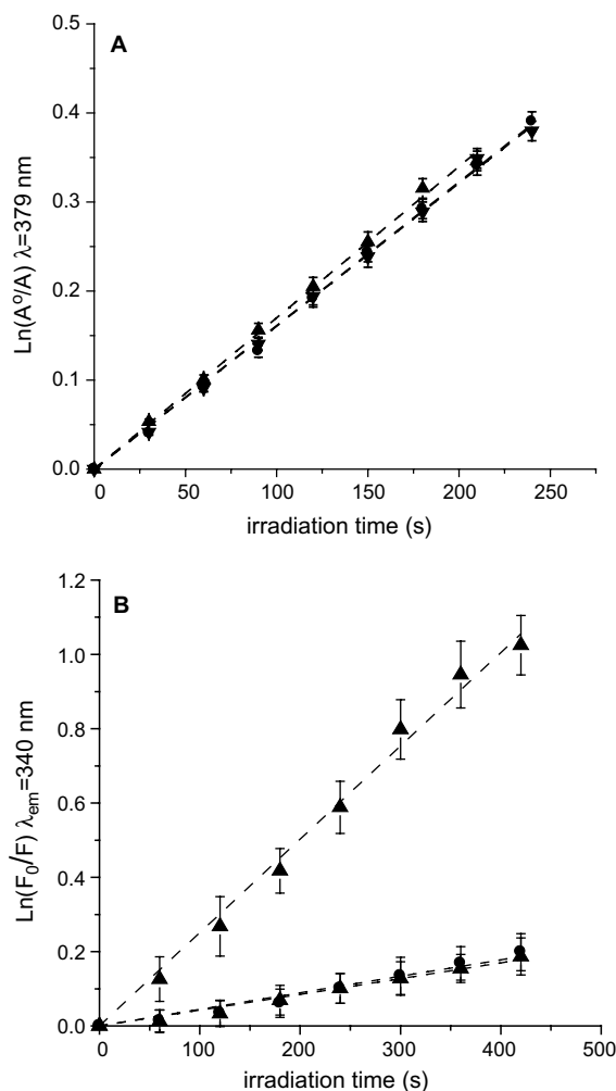
Figure 2. First-order plots for the photooxidation of (A) DMA (35 \mu\text{M} ) and (B) Try (25 \mu\text{M} ) photosensitized by ZnPc 1 (▼), ZnPc 2 (▲), and ZnPc (●) in DMF; \lambda_{\text{irr}} = 590\text{--}800 \text{ nm} . Values represent means \pm standard deviation of three separate experiments.
