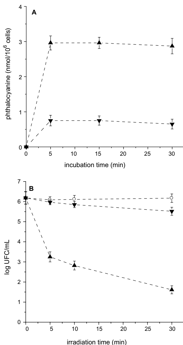
Figure 4. (A) Amount of ZnPcs 1 ( \blacktriangledown ) and 2 ( \blacktriangle ) recovered after one washing step from E. coli cells treated with 10 \mu\text{M} of sensitizer for different incubation times, at 37 °C in the dark. (B) Survival curves of E. coli incubated with 10 \mu\text{M} of ZnPcs 1 ( \blacktriangledown ) and 2 ( \blacktriangle ) for 30 min at 37 °C in the dark, washing once before illumination and exposed to visible light for different irradiation times. Values represent means \pm standard deviation of three separate experiments.
