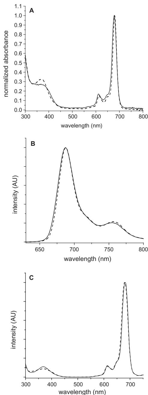
Figure 1. (A) Absorption spectra; (B) fluorescence emission spectra, \lambda_{\text{exc}} = 612 nm; and (C) fluorescence excitation spectra, \lambda_{\text{em}} = 760 nm, of ZnPc 1 (---) and ZnPc 2 (—) in DMF.
