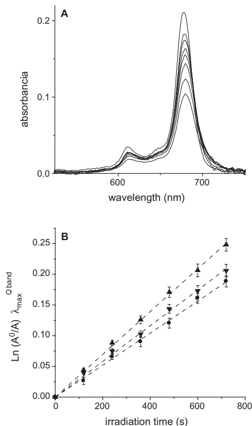
Figure 3. (A) Absorption spectra changes of ZnPc 2 irradiated with visible light in DMF ( \Delta t = 10 min). (B) First-order plots for the photobleaching of ZnPc 1 ( \blacktriangledown ), ZnPc 2 ( \blacktriangle ), and ZnPc ( \bullet ) in DMF irradiated with visible light. Values represent means \pm standard deviation of three separate experiments.
